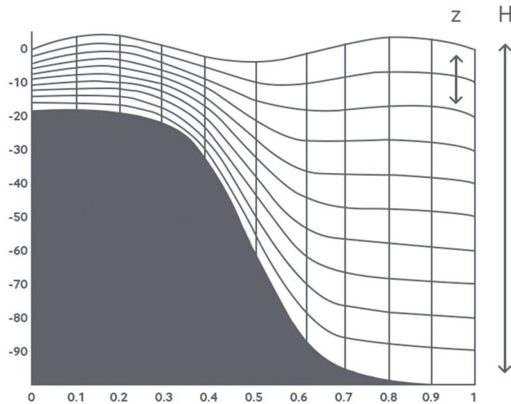
Figure 2-2. Schematic of the BFHYDRO vertical sigma coordinate system.
