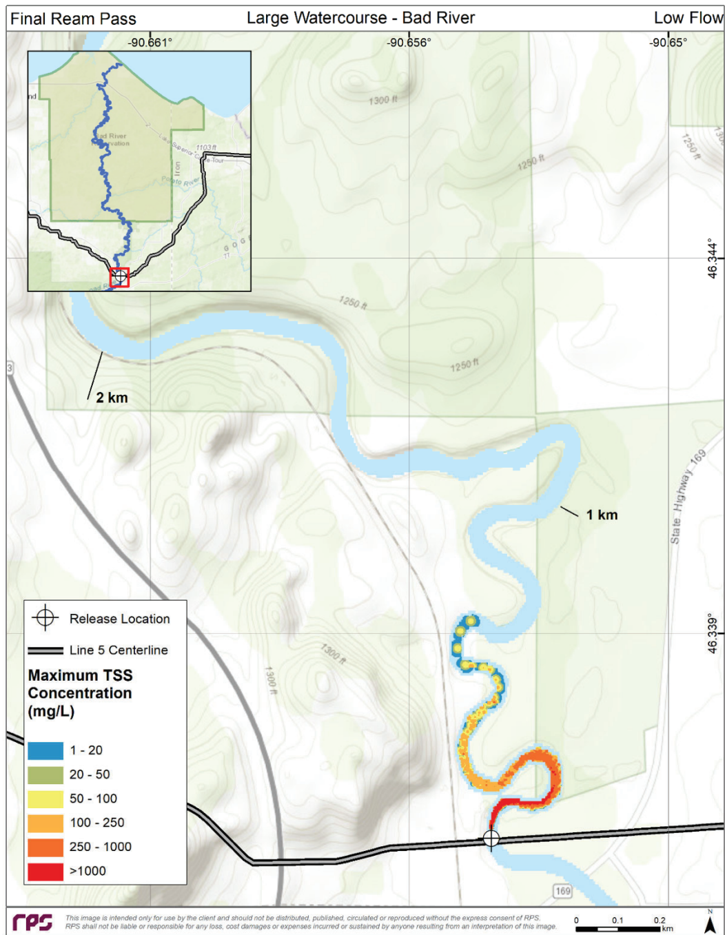
Figure 5-6. Maximum TSS concentrations above background predicted at any time in the simulation for the Final Ream Pass scenario in low flow conditions. Downstream distance is provided on the map for reference (1 km = 0.62 miles; 2 km = 1.24 miles).
